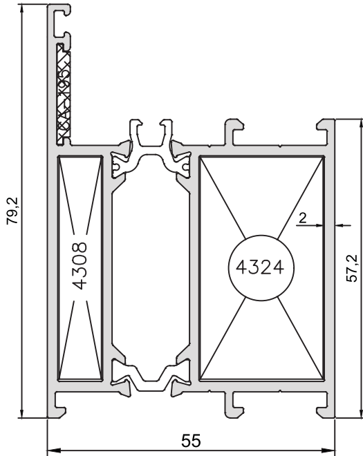
KOD-CODE AT-5513-20 TEORİK AĞIRLIK THEORETICAL WEIGHT 1,875 Kg/m
