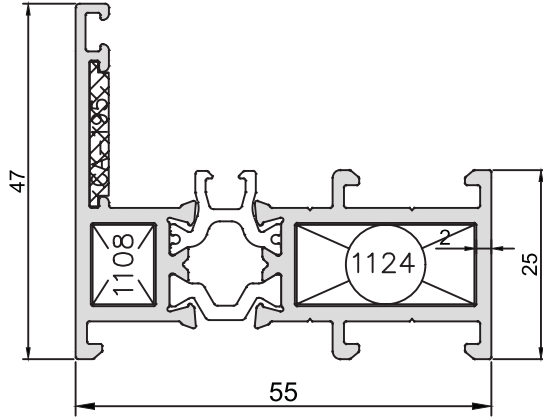
KOD-CODE AT-5511-20 TEORİK AĞIRLIK THEORETICAL WEIGHT 1,198 Kg/m
