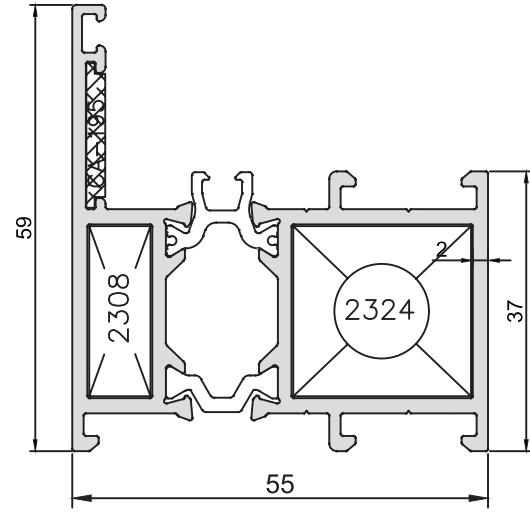
KOD-CODE AT-5512-20 TEORİK AĞIRLIK THEORETICAL WEIGHT 1,458 Kg/m
